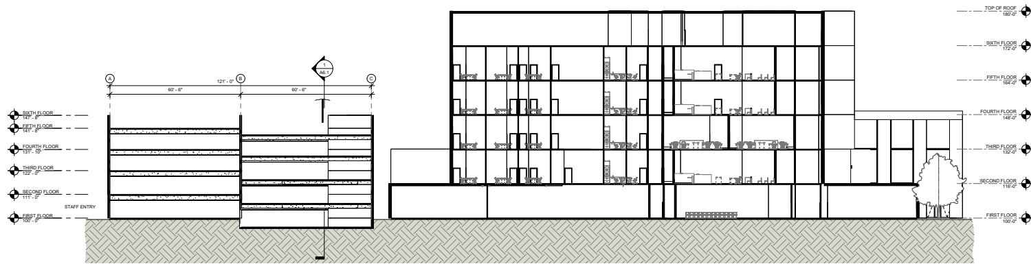
2 BUILDING SECTION - GARAGE & JUSTICE CENTER SCALE: 1/8" = 1'-0"
