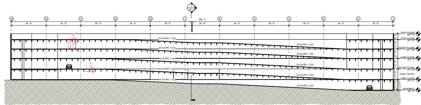
1 PARKING GARAGE SECTION SCALE: 1/8" = 1'-0"
